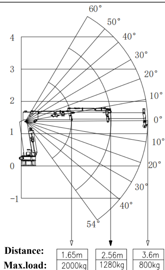
Boom working range diagram
